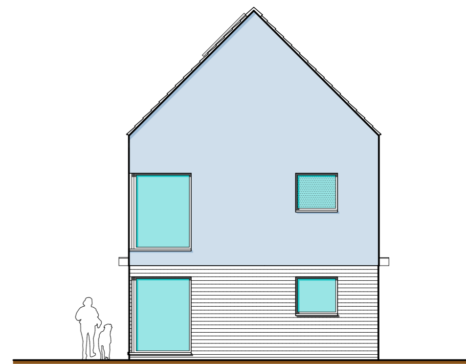
PROPOSED SIDE ELEVATION - [SEALAND AVENUE - NORTH EAST]
